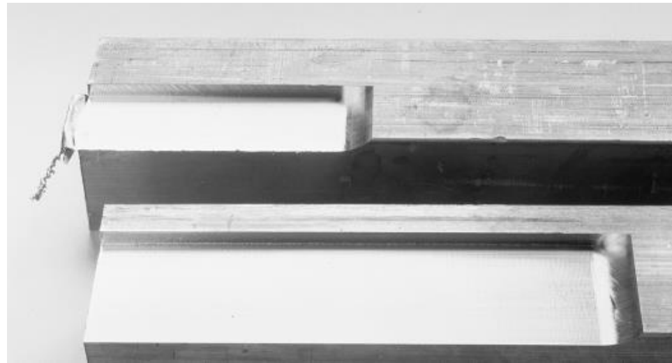
Top – Regular copper with characteristic burr; Bottom - Tellurium Copper
